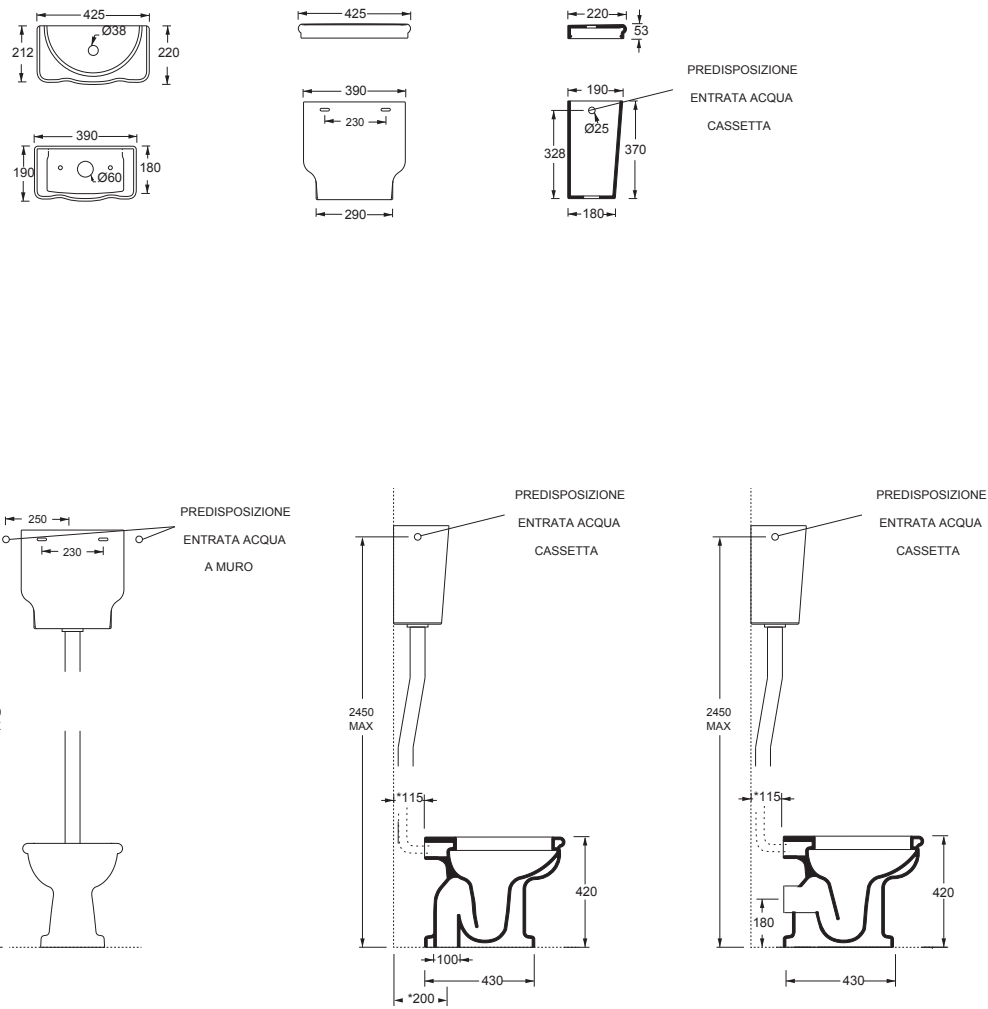
Cassetta alta meccanismo non incluso High cistern. flushing mechanism not included
