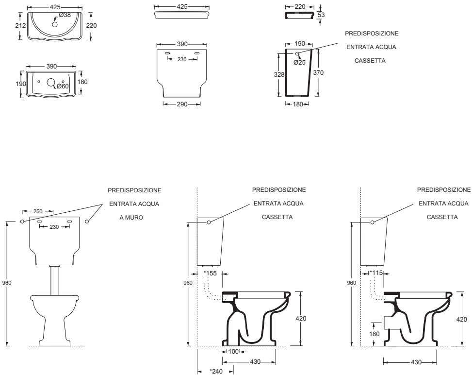
Cassetta a zaino meccanismo non incluso Low level flushing mechanism not included
